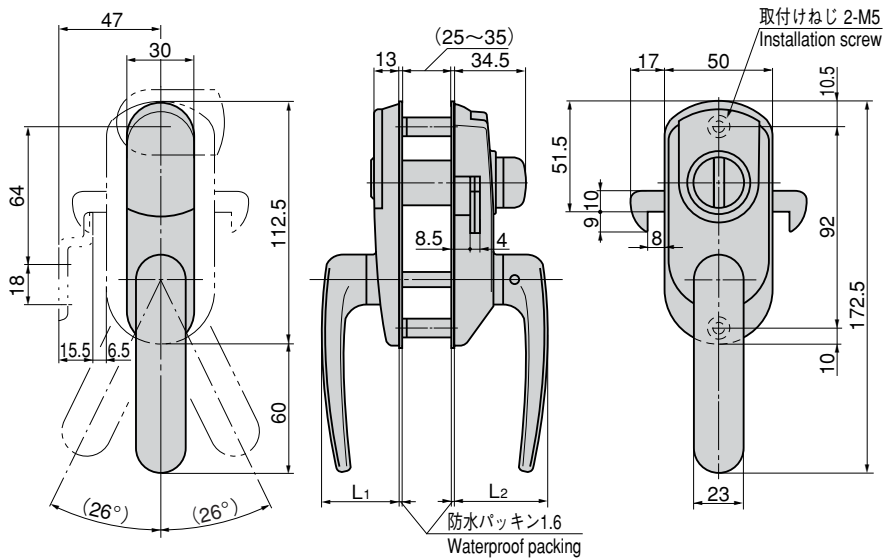
A-298-HS (表) (Front)
