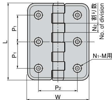
BP-14-12-S 皿ねじ用 For countersink screw
