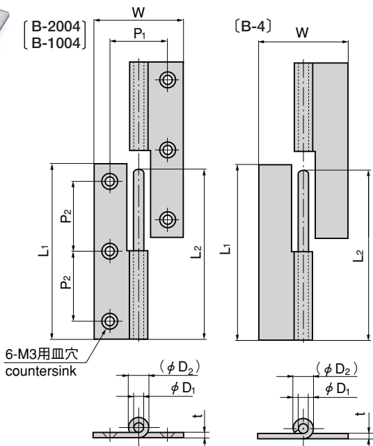
B-1004-1-R (ステンレス製の標準は穴あきです) Standard of stainless steel-made is supplied with hole.
