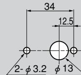
パネル穴明け寸法 (本体側) Panel drilling dimensions (Main body)
