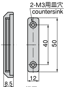
[C-74用受け金具] base plate
