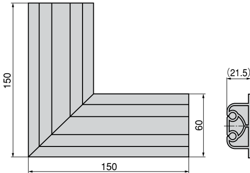
〔FC-784〕保冷車用ゴム 長さ2.5m Rubber for cold storage vehicle
