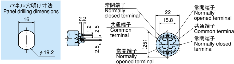
(2回路2接点型の裏面) (Back of two-circuit-two-contact type)
